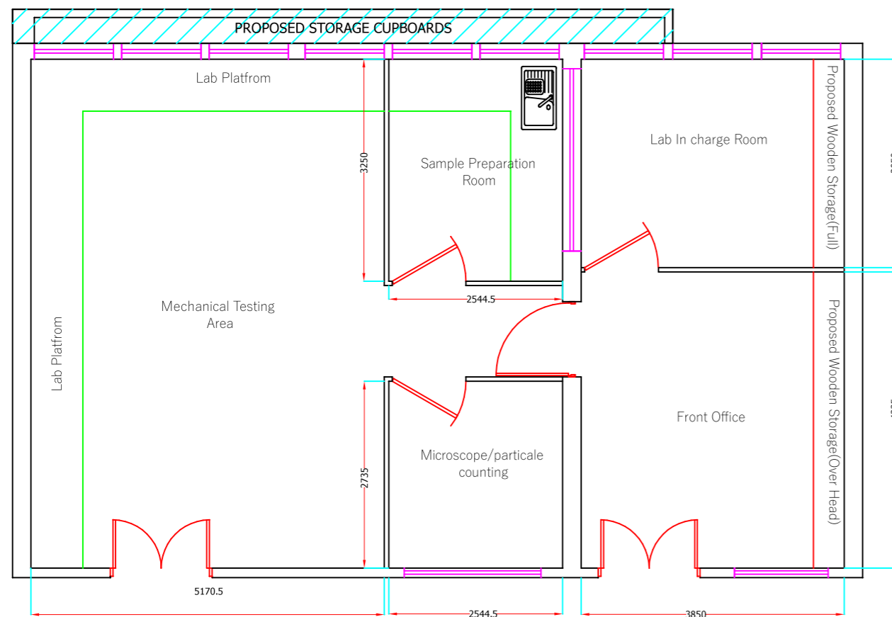
PROPOSED NEW METALLURGY LAB LAYOUT
