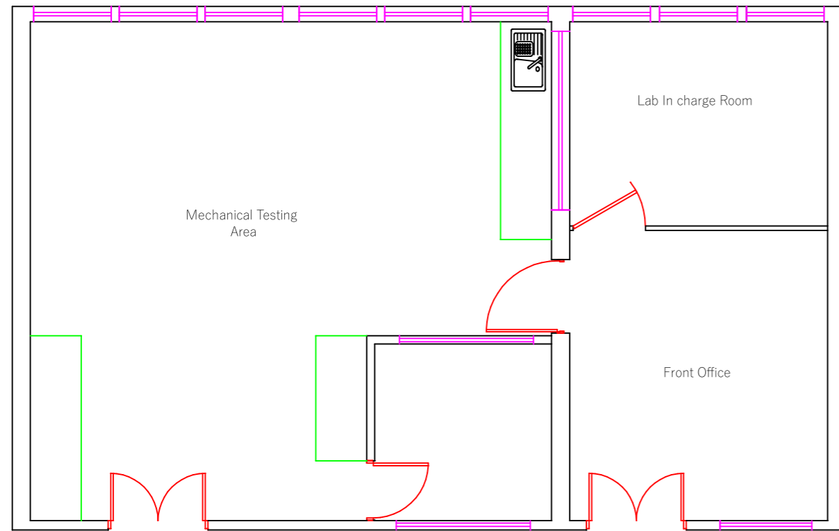
EXISTING METALLURGY LAB LAYOUT
