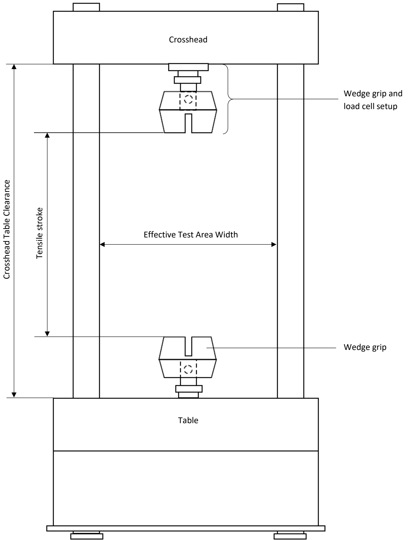
Figure 1: Schematic Diagram of Universal Testing Machine marking the nomenclatures used in Tender document
